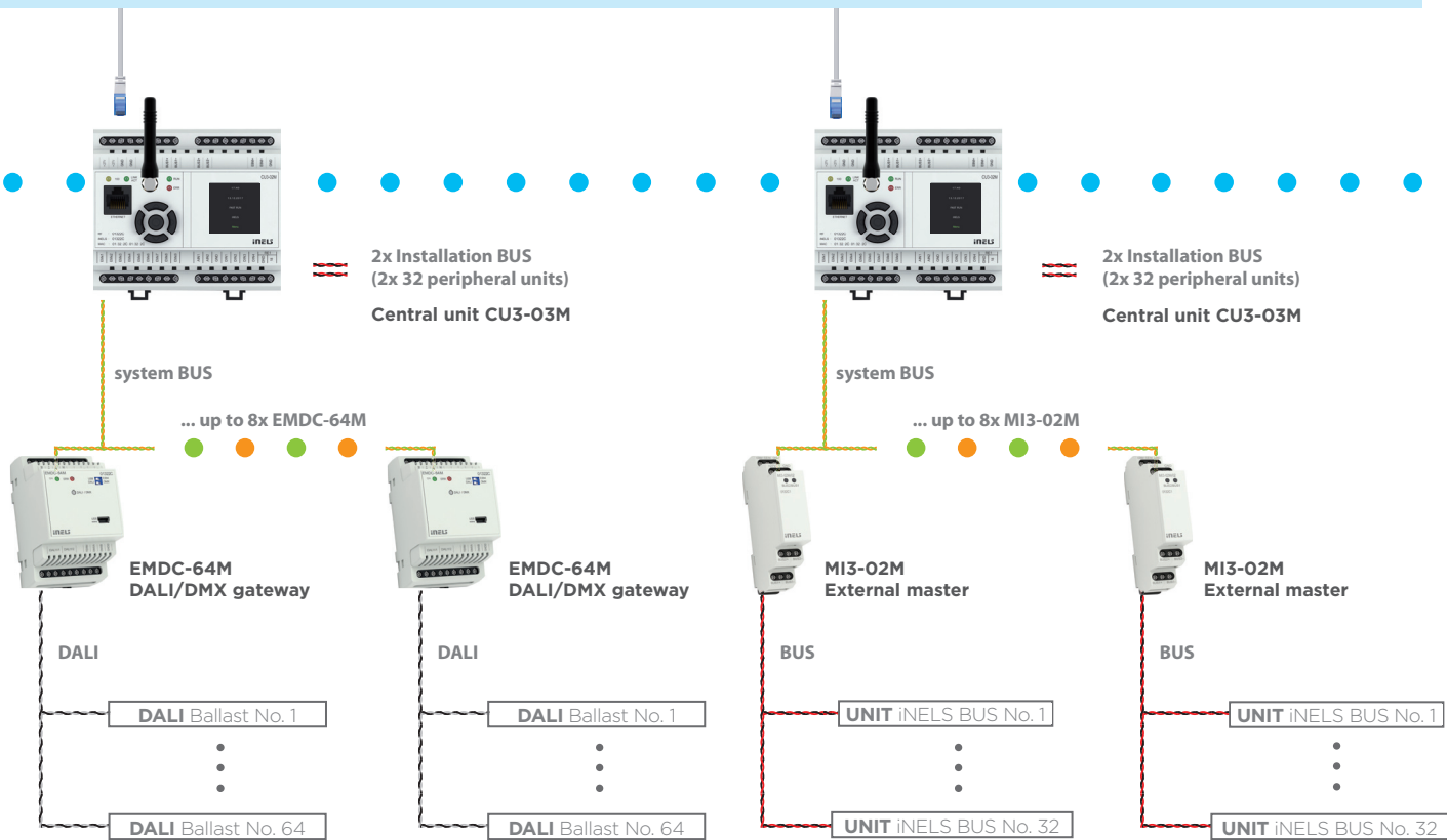
iNELS BMS
