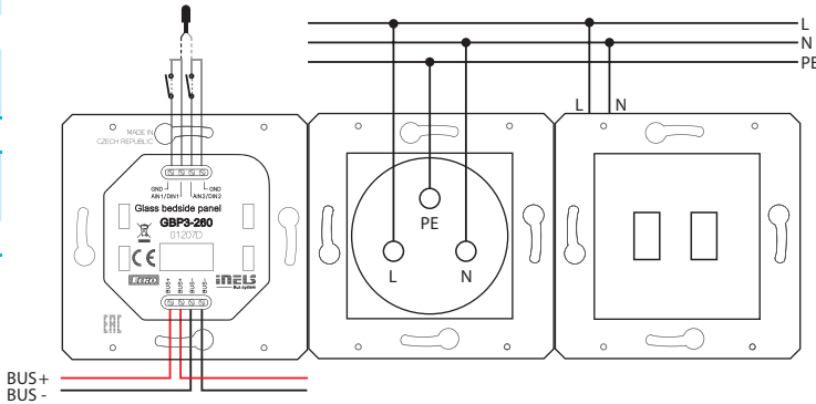
GBP3-260/xR/2F-23x-20x
