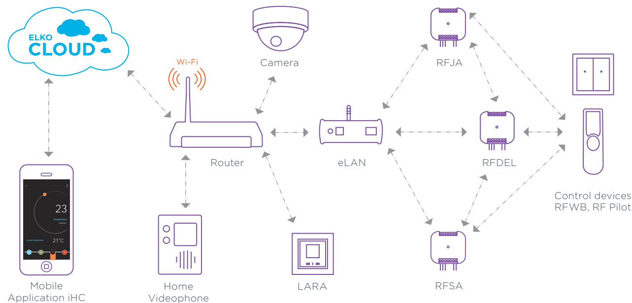
Functional diagram RFIO
