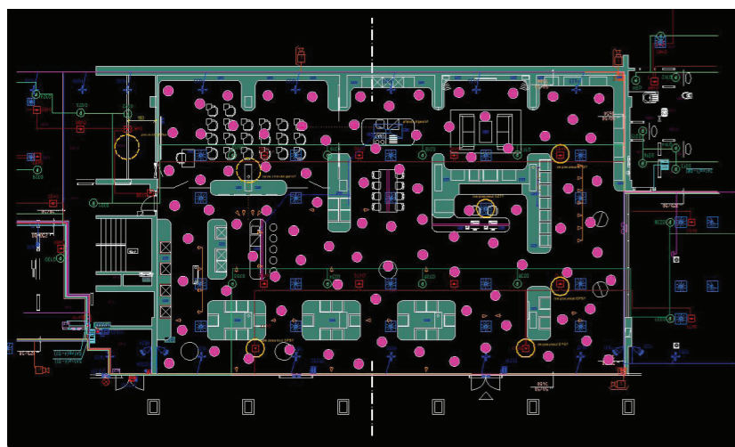
FLOORPLAN OF SHOWROOM DIAMOND DESIGN PRAHA
