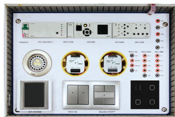
input/output points
