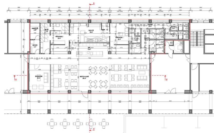
FLOORPLAN OF SHOWROOM INELS CAFÉ
