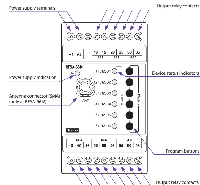
RFSA-66MI/230V RFSA-66M/230V
