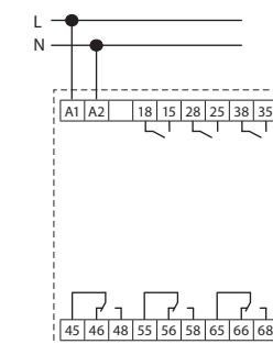
RFSA-66MI/230V RFSA-66M/230V
